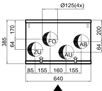
EA180.6 Bypass links
