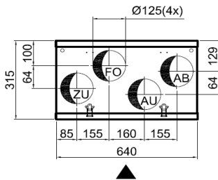
EA180.6 Basis links
