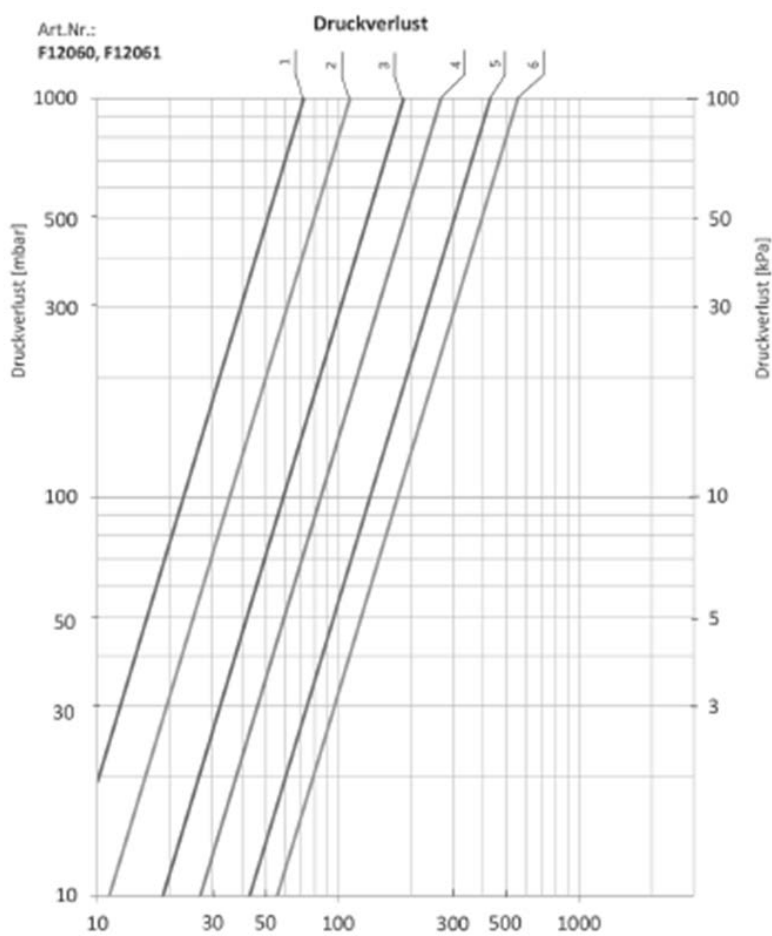
Fig. 3: Pressure drop diagram
