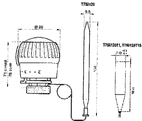
Fig. 1. Thera-2080WL with remote sensor
